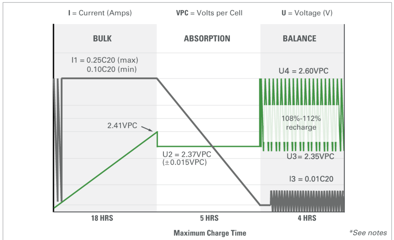
Constant Current (IUI) Charge Profile
