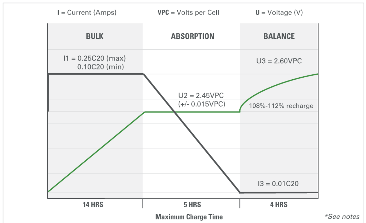
Voltage Regulated (IUI) Charge Profile
